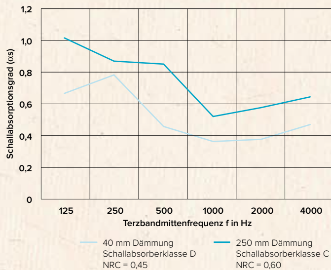
ATMOphon EASYLINE 20/40/40
