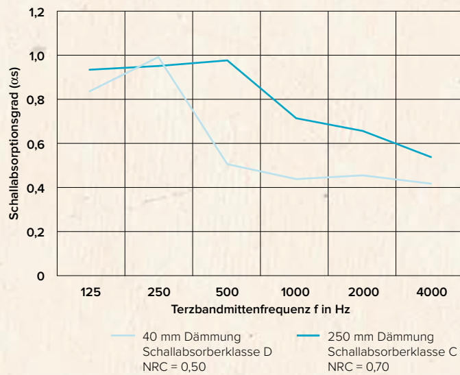
ATMOphon EASYLINE 20/58/20
