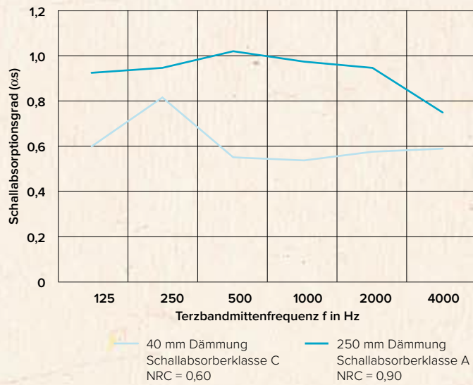
ATMOphon EASYLINE 25/25/50
